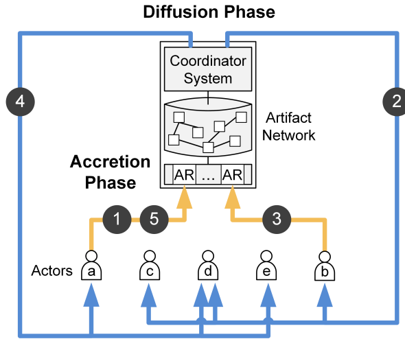
Figure 2: Characteristic SIS process with alternating accretion phase (yellow) and diffusion phase (blue).
